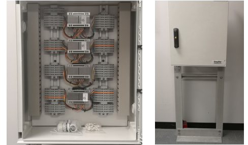
GBK4383 4 Aspect LEU Dis Box GBK4384 GRP Mounting Assembly
